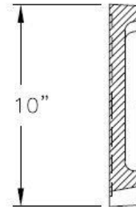
COVER SECTION
